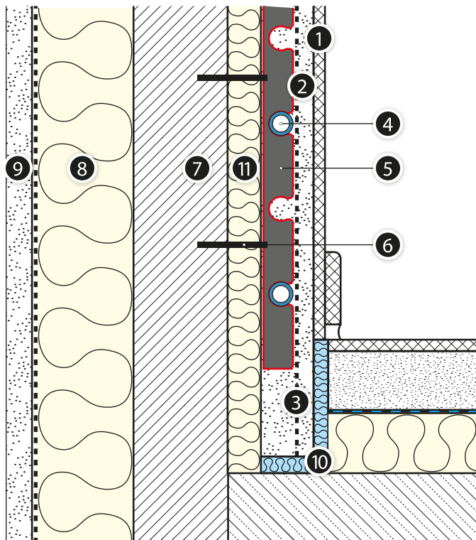
Fig. 32. KAN-therm TBS Rail heating/cooling structure
