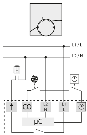
Fig. 64. Clamps and Basic 230 or 24V heating/cooling thermostat connection diagram (with an option of periodic temperature lowering by connecting a clock)
