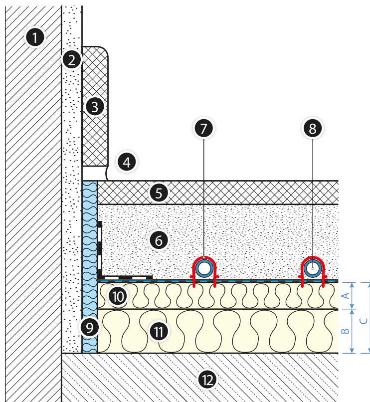
Fig. 22. Floor heater with KAN-therm Tacker System board and supplementary insulation on the ceiling above internal not heated room and on the ceiling in contact with outside air
