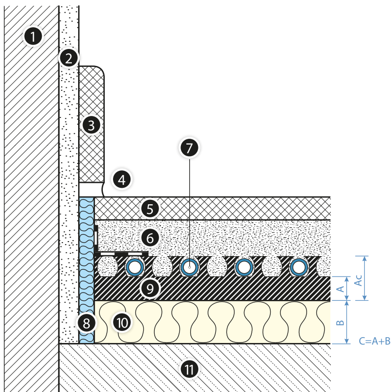
Fig. 26. Floor heater with KAN-therm Profil System board and supplementary insulation on the ceiling above internal not heated room and on the ceiling in contact with outside air
