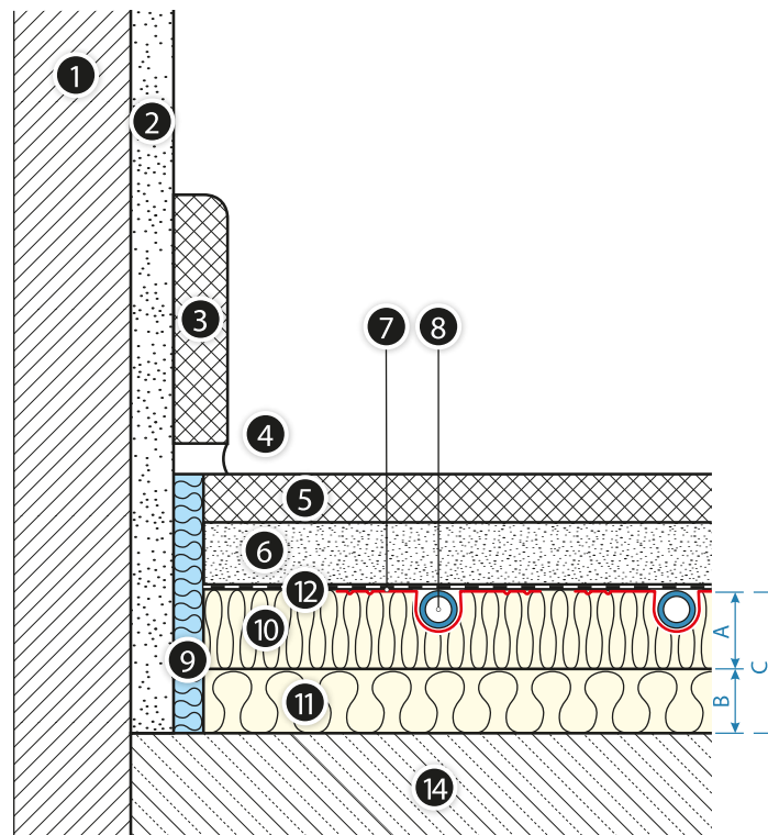
Fig. 29. Floor heater with KAN-therm TBS System board and supplementary insulation on the ceiling above internal room and on the ceiling in contact with outside air
