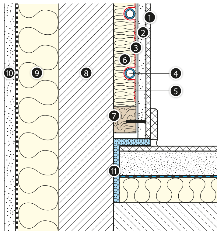
Fig. 34. KAN-therm TBS Wall heating/cooling structure
