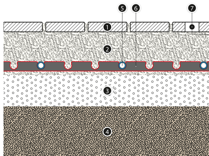
Fig. 39. External traffic routes heating (KAN-therm Rail System)
