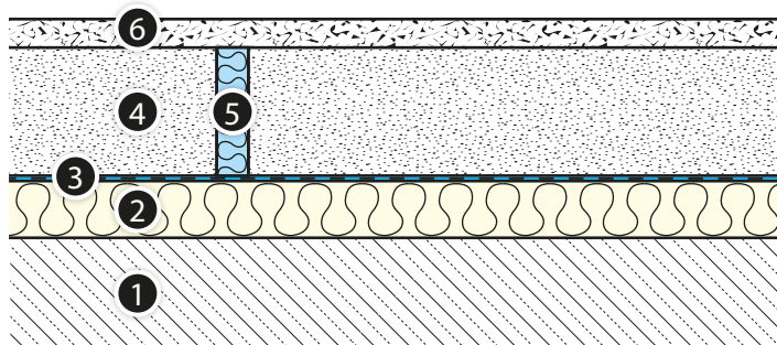
Fig. 14. Performance of dilatation gap in case of flooring made of soft covering.
