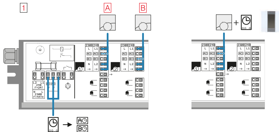
Fig. 70. Time control devices connection
