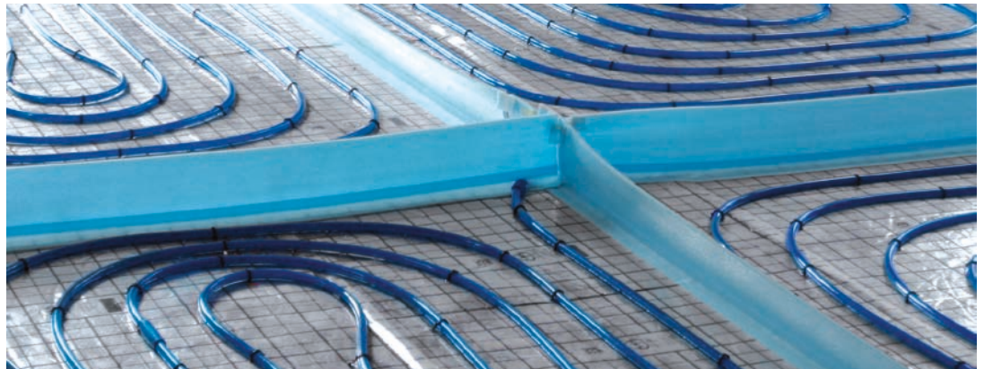
Fig. 13. Distribution of heating fields with dilatation gaps
