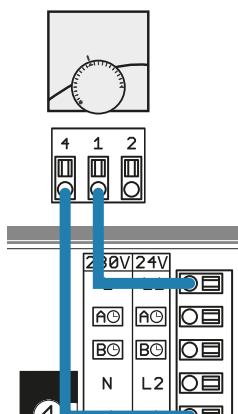
Fig. 62. Clamps and 24 – 230V (0.6107) bimetallic thermostat connection to the Basic electrical terminal block diagram
