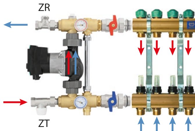
Fig. 61. K-803003 (or K-803000, K-803001) pump group with 75A (or 71A, 55A, 51A) manifold - flow directions
