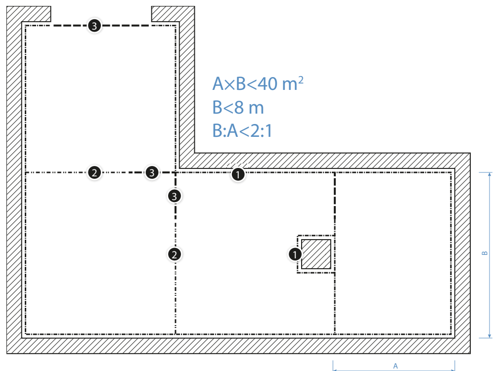
Fig. 17. Heating pipes dilatation in floor heating rules of performance
