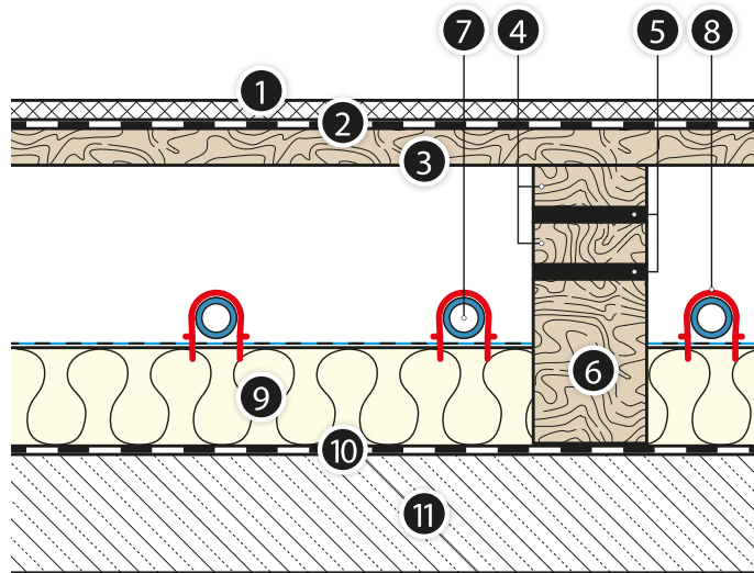
Fig. 37. Cross-section of the floor with surface elasticity, with a floor heating installation made of KAN-therm Tacker System elements.
