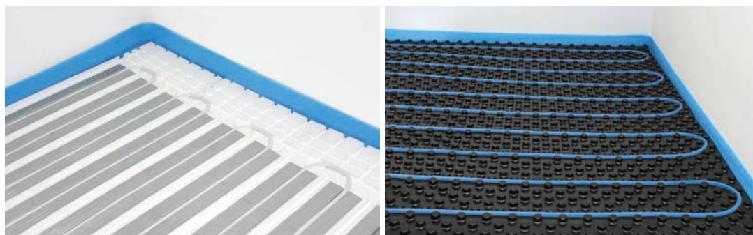
Fig. 12. Examples of edge insulation in KAN-therm floor heating.
