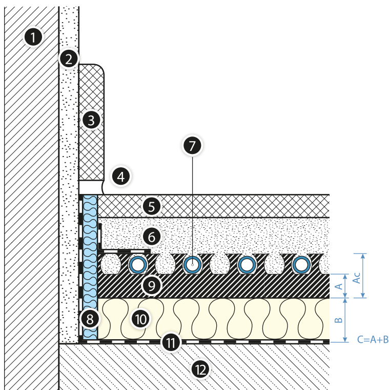
Fig. 28. Floor heater with KAN-therm Profil System board and supplementary insulation and damp-proof coating on the ceiling laid out on the ground
