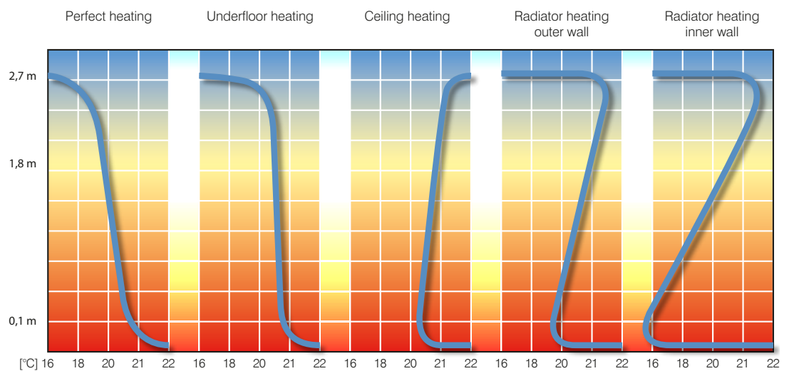
Fig. 1. Vertical temperature distribution for various types of heating
