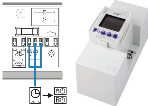
Fig. 76. Clock to Basic terminal block connection diagram
