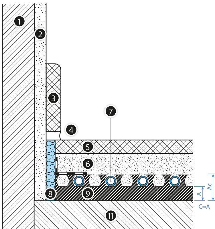
Fig. 25. Floor heater with KAN-therm Profil System board on the ceiling above an internal room
