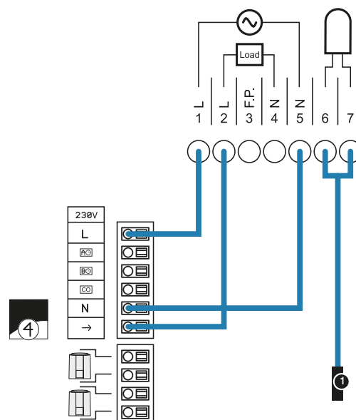
Fig. 66. Clamps and TH232-AF week thermostat connection diagram
