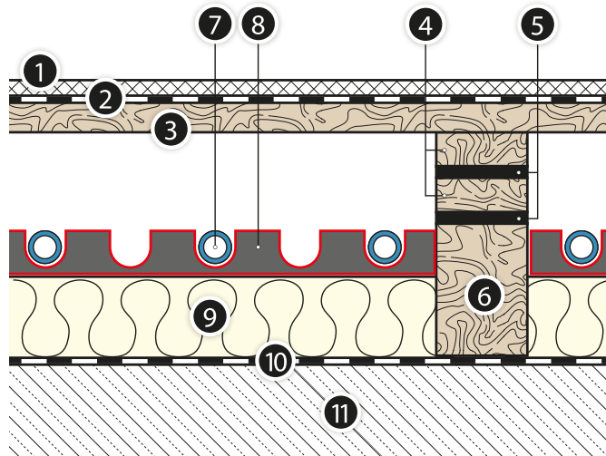
Fig. 38. Cross-section of the floor with surface elasticity, with a floor heating installation made of KAN-therm Rail System elements.
