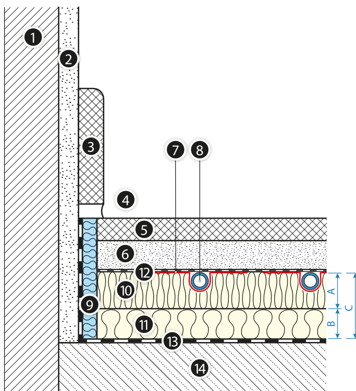
Fig. 30. Floor heater with KAN-therm TBS System board and supplementary insulation and damp-proof coating on the ceiling laid out on the ground
