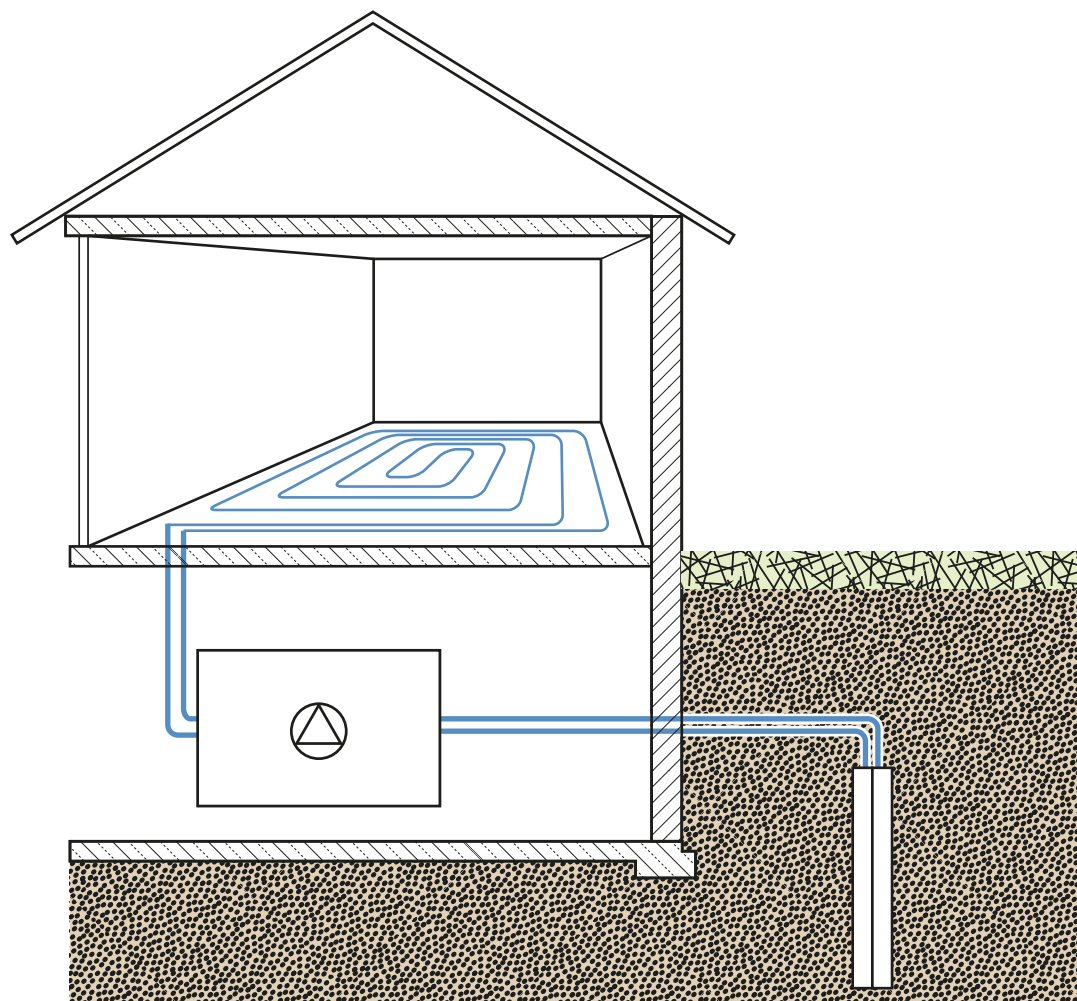
Fig. 2. Surface heating installation supply directly from low-temperature heat source
