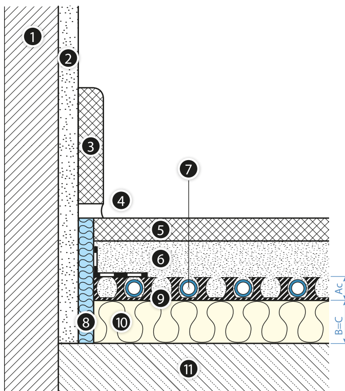
Fig. 27. Floor heater with KAN-therm Profil3 System board and supplementary insulation on the ceiling above the internal not heated room and on the ceiling laid out on the ground (damp insulation required!)
