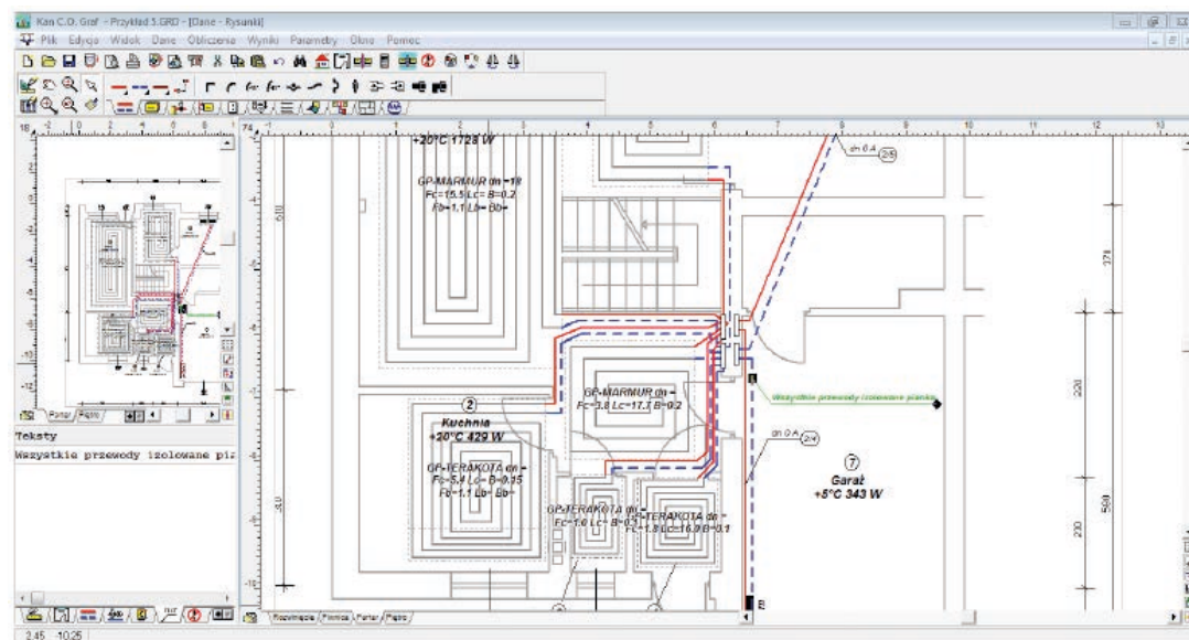
Fig. 81. Floor plan with projected floor heaters.
