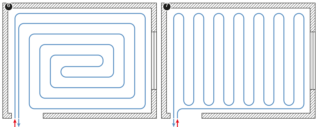
Fig. 6. Floor heating/cooling coil in spiral pattern.
