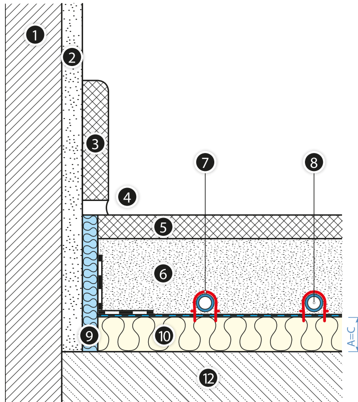
Fig. 21. Floor heater with KAN-therm Tacker System board on the ceiling above an internal room
