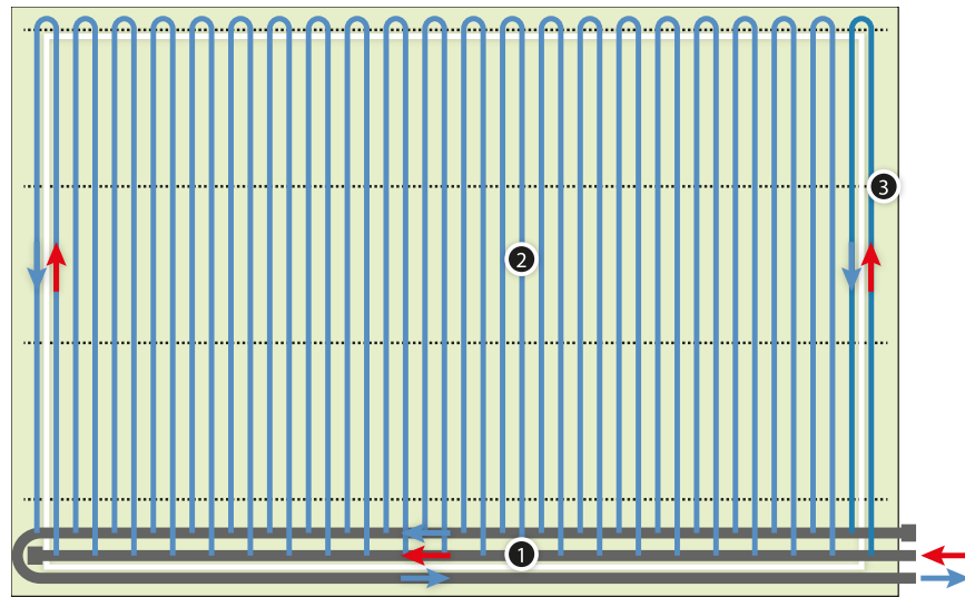
Fig. 42. KAN-therm field pitch heating installation – flowchart
