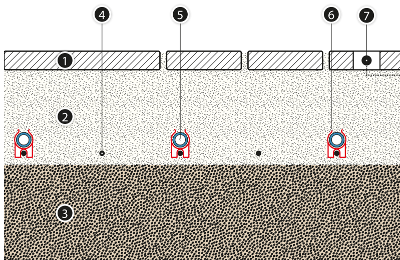
Fig. 40. External traffic routes heating (KAN-therm NET System)
