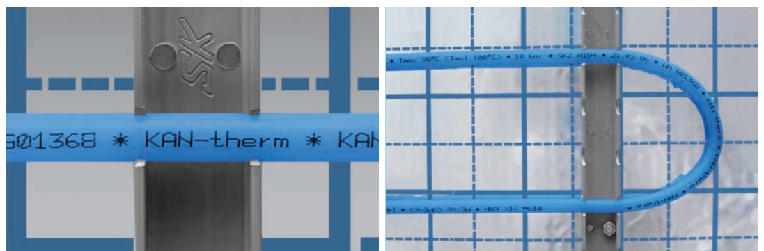
Fig. 33. KAN-therm heating pipes mounting in wall heating performed using wet method
