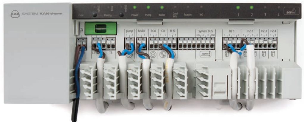
Fig. 74. Transparent and clear signalisation of terminal block work status, simple and secure connection of actuators to external devices
