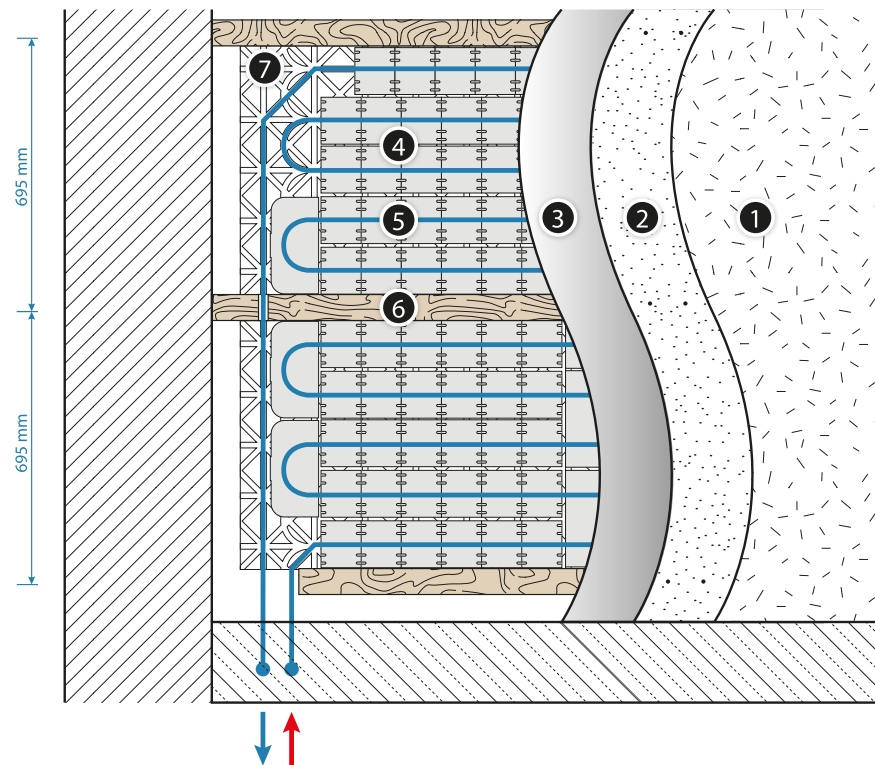
Fig. 35. KAN-therm TBS Wall heating/cooling structure
