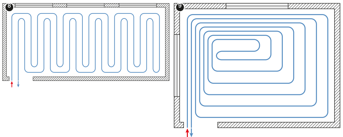
Fig. 8. Floor heating/cooling coil in mixed arrangement: double series pattern.
