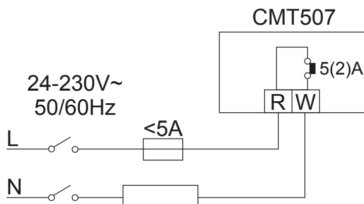
Fig. 65. Clamps and 24 – 230V week regulator connection to Basic electrical terminal block diagram
