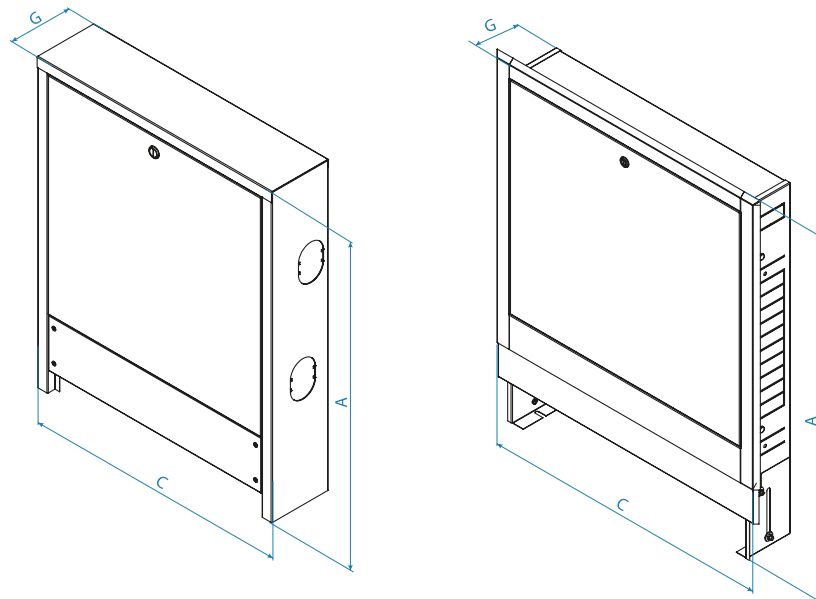
Fig. 52. KAN-therm installation cabinet dimensions
