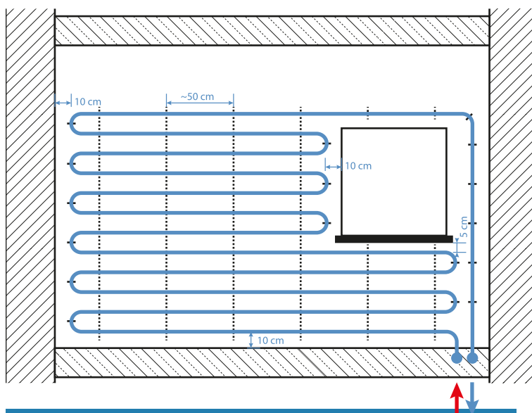
Fig. 31. Mounting distance in wall heating
