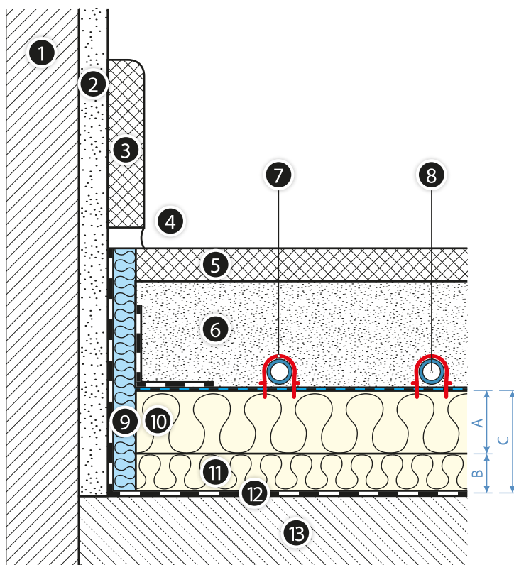
Fig. 23. Floor heater with KAN-therm Tacker System board and supplementary insulation and damp-proof coating on the ceiling laid out on the ground
