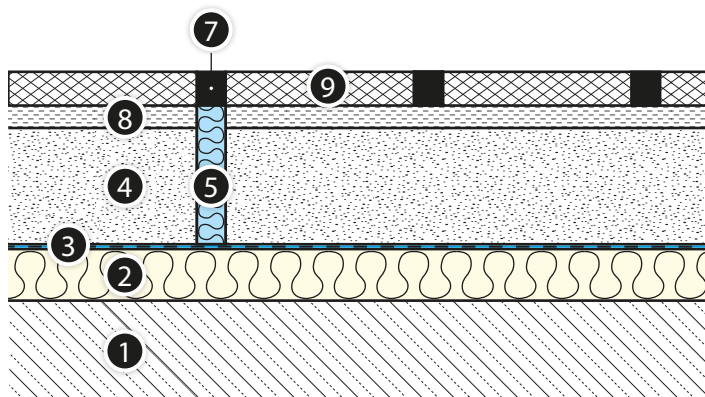
Fig. 15. Performance of dilatation gap in case of stone flooring
