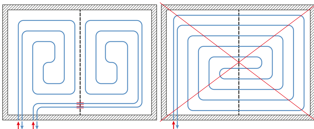
Fig. 18. Correct and incorrect distribution of heating field with a dilatation gap
