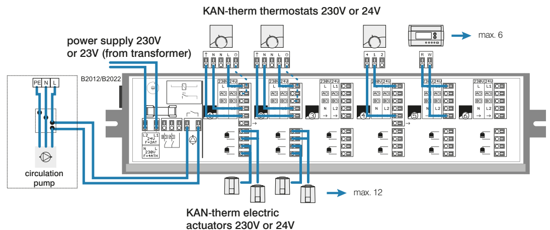
Fig. 68. Basic 240V or 24V electrical terminal block with pump module configuration
