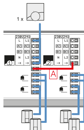
Fig. 69. 3 or 4 controlled by single thermostat actuators connection
