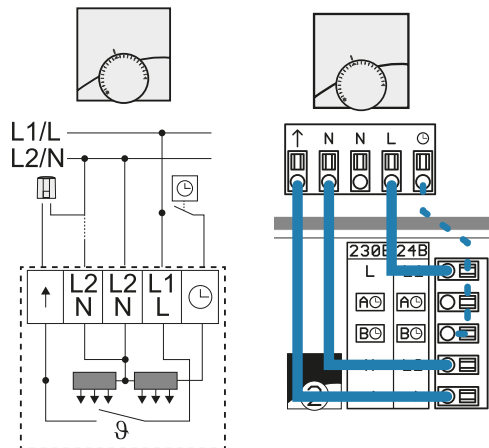
Fig. 63. Clamps and Basic 230 or 24V thermostat connection to Basic electrical terminal blocks diagram (with an option of periodic temperature lowering through connection of a clock)
