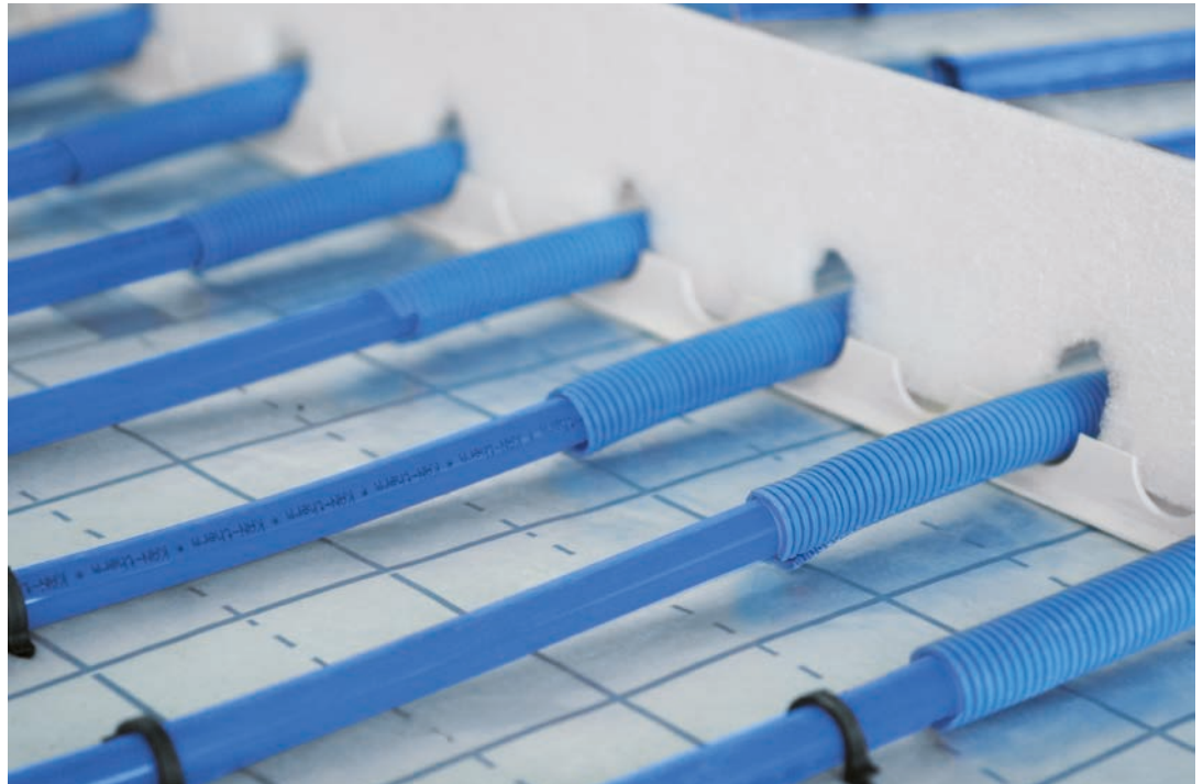
Fig. 16. Dilatation profile - way of transit pipes arrangement through dilatation
